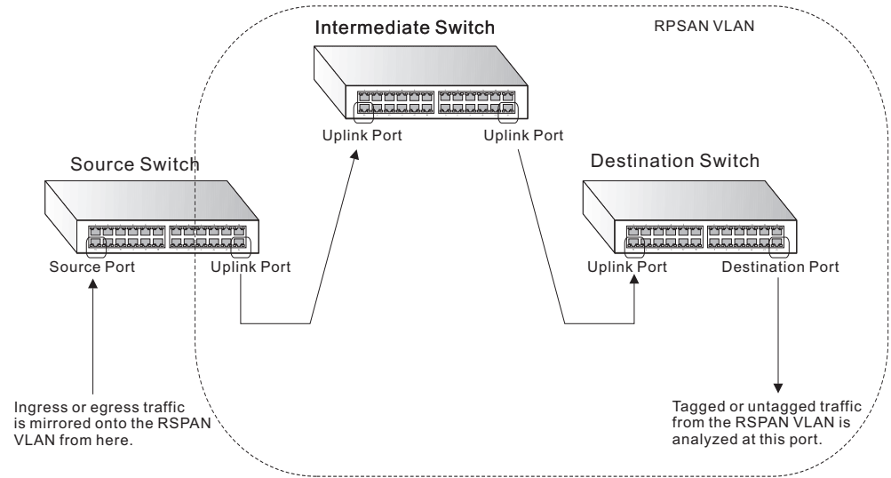
Figure 93: Configuring Remote Port Mirroring
