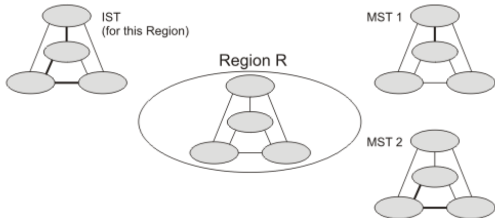
Figure 48: MSTP Region, Internal Spanning Tree, Multiple Spanning Tree
