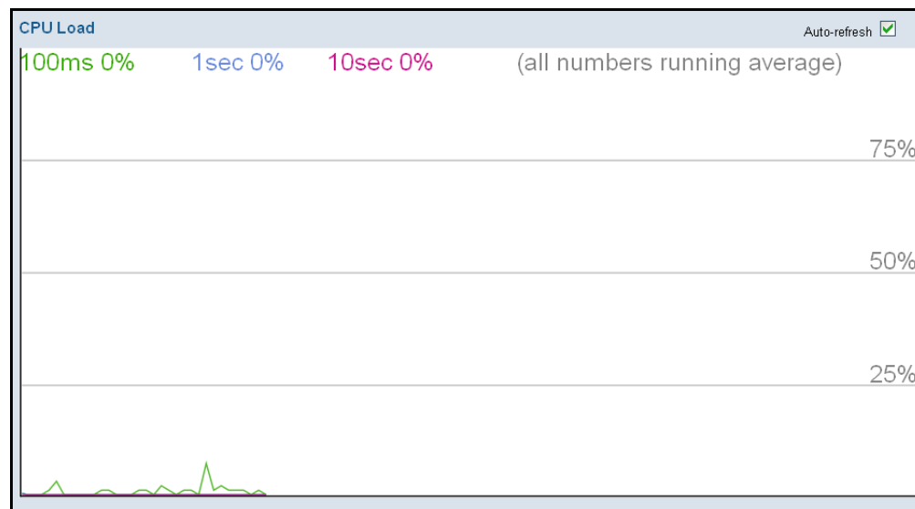
Figure 100: CPU Load
