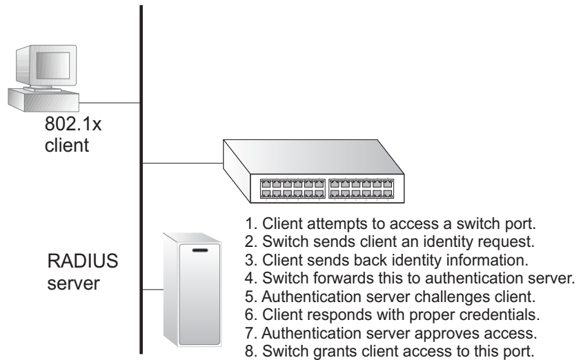
Figure 32: Using Port Security
