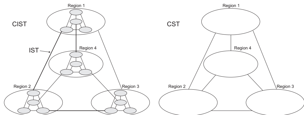
Figure 49: Common Internal Spanning Tree, Common Spanning Tree, Internal Spanning Tree
