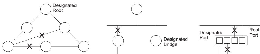
Figure 47: STP Root Ports and Designated Ports
